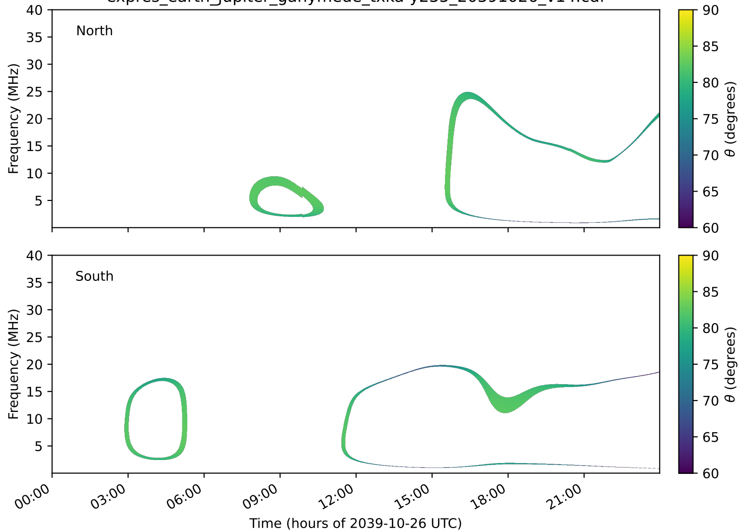
expres_earth_jupiter_ganymede_txka-y235_20391026_v14.cdf
