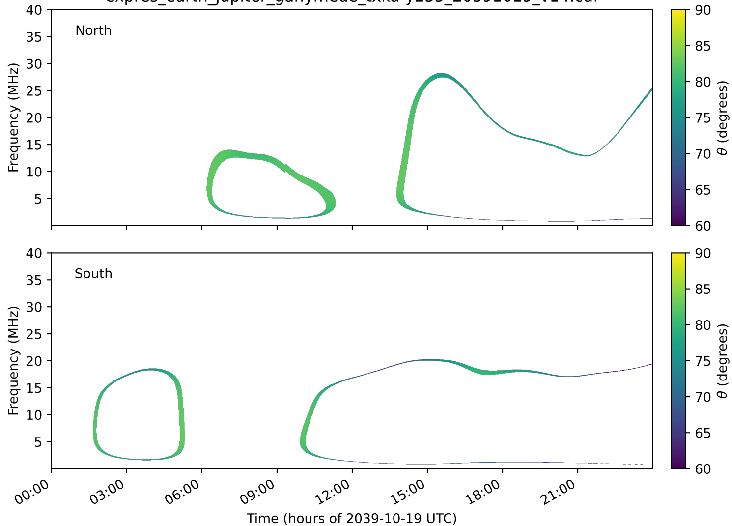
expres_earth_jupiter_ganymede_txka-y235_20391019_v14.cdf
