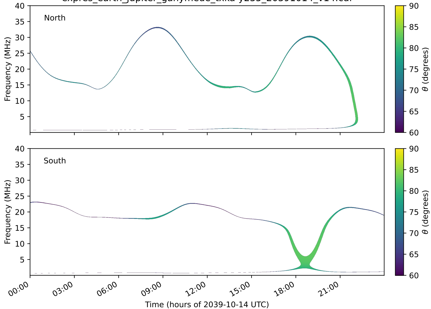
expres_earth_jupiter_ganymede_txka-y235_20391014_v14.cdf
