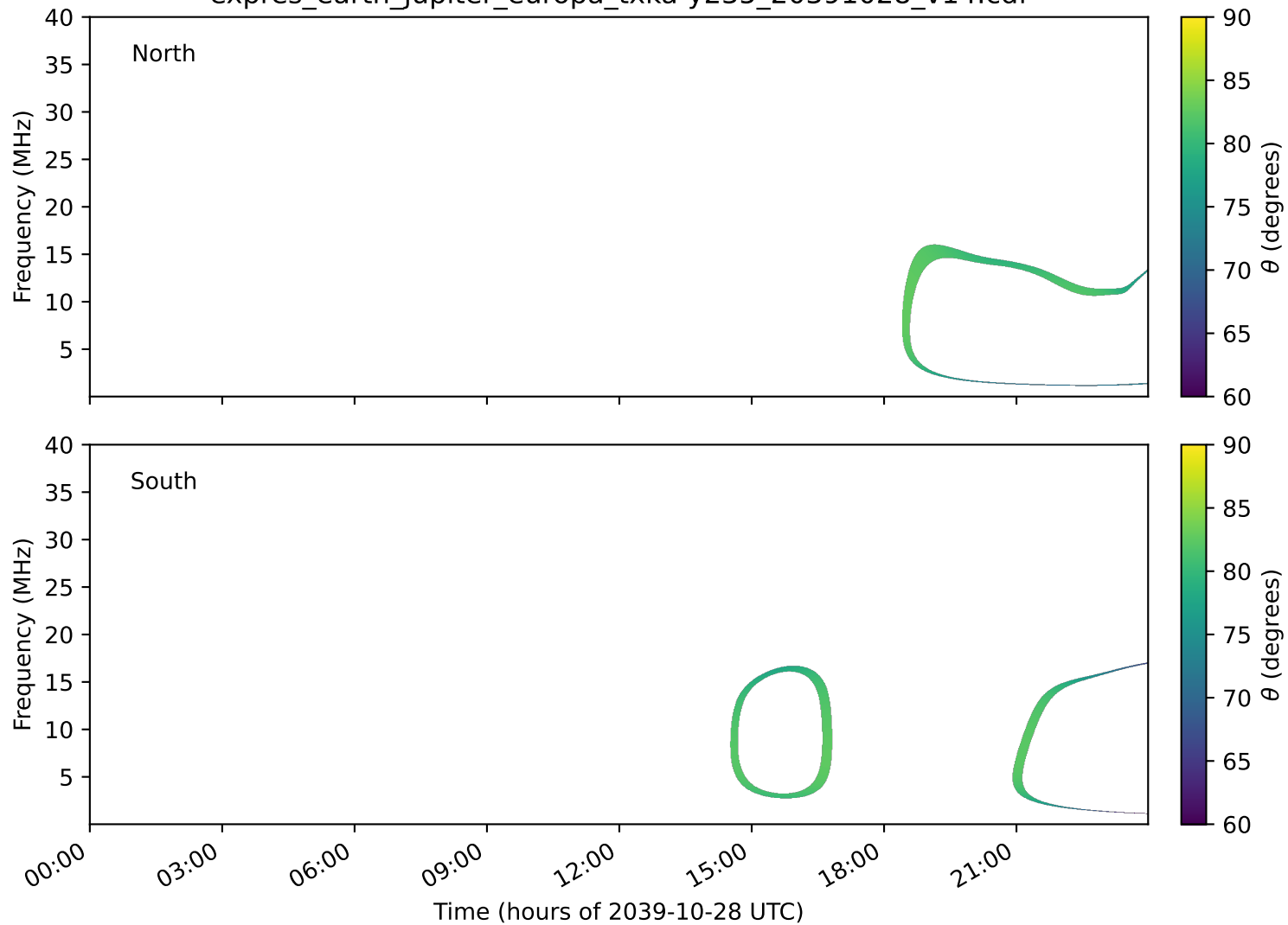
expres_earth_jupiter_europa_txka-y235_20391028_v14.cdf
