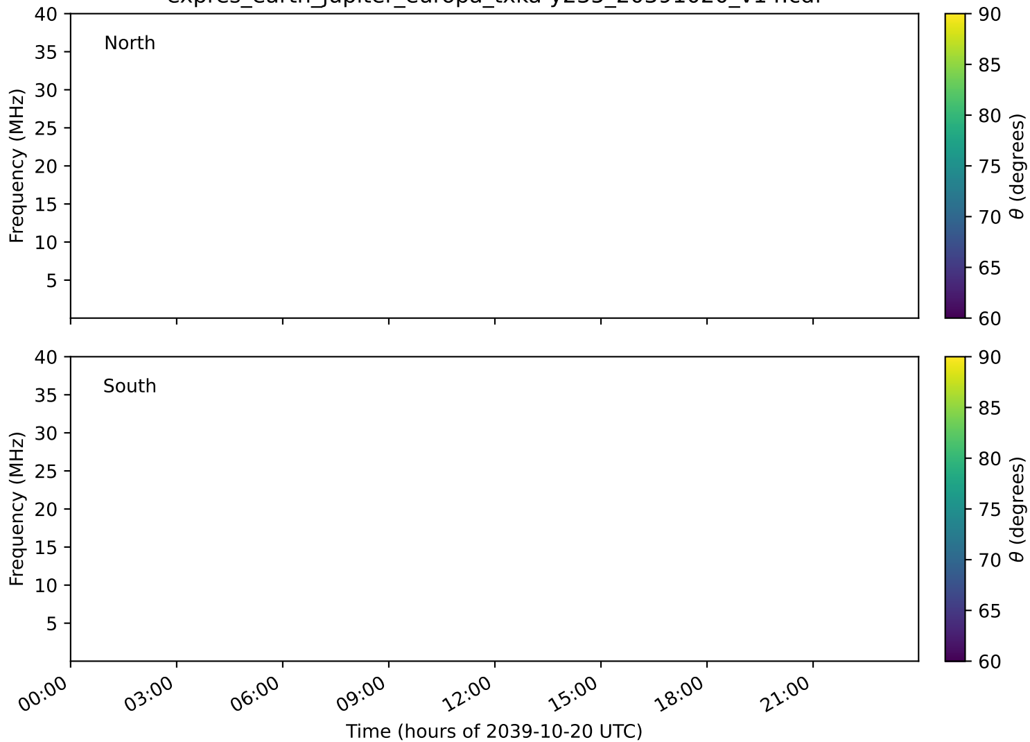
expres_earth_jupiter_europa_txka-y235_20391020_v14.cdf
