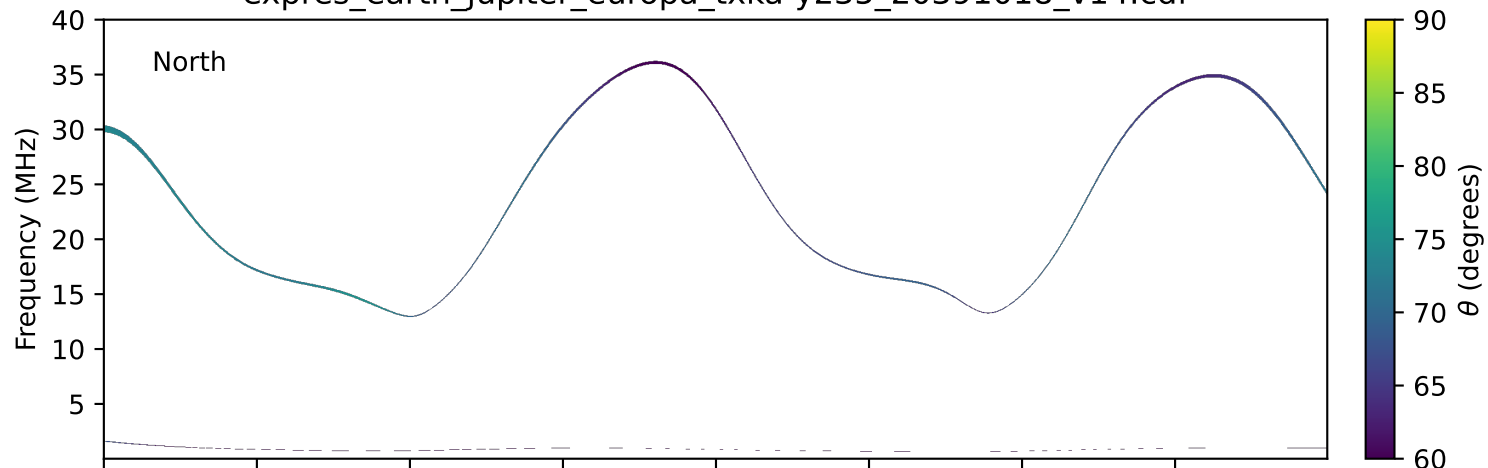
expres_earth_jupiter_europa_txka-y235_20391018_v14.cdf
