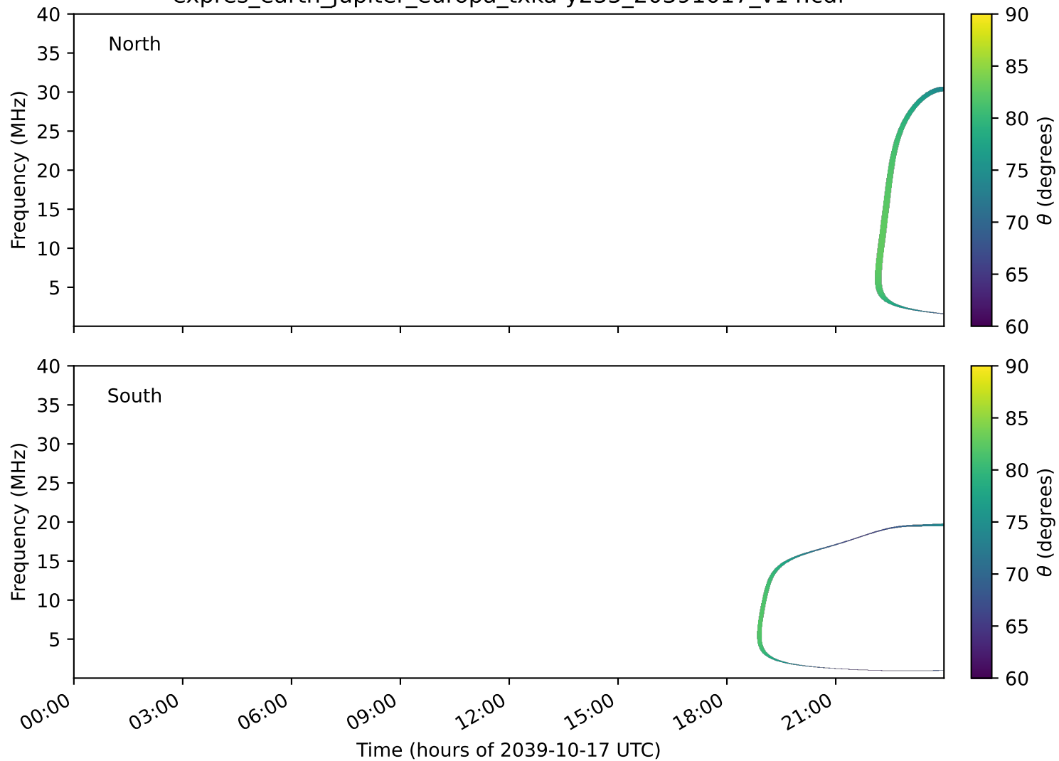
expres_earth_jupiter_europa_txka-y235_20391017_v14.cdf
