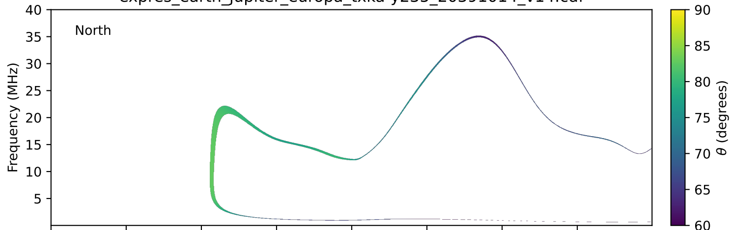
expres_earth_jupiter_europa_txka-y235_20391014_v14.cdf
