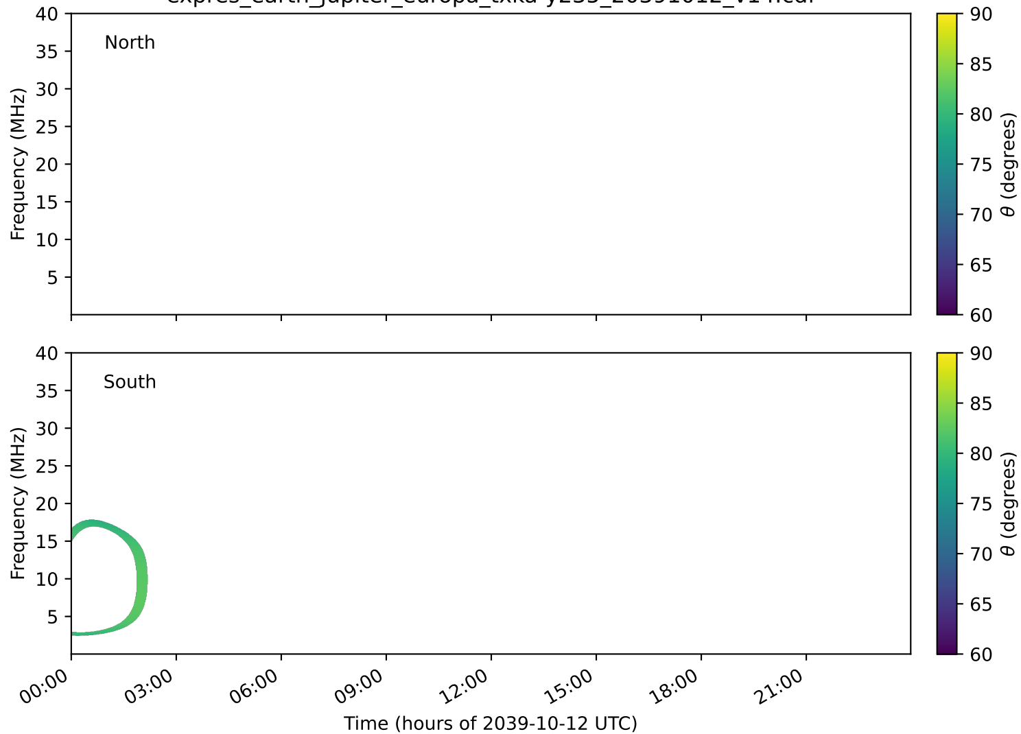
expres_earth_jupiter_europa_txka-y235_20391012_v14.cdf
