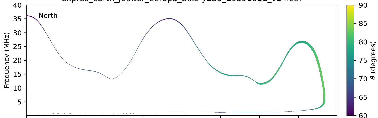
expres_earth_jupiter_europa_txka-y235_20391011_v14.cdf
