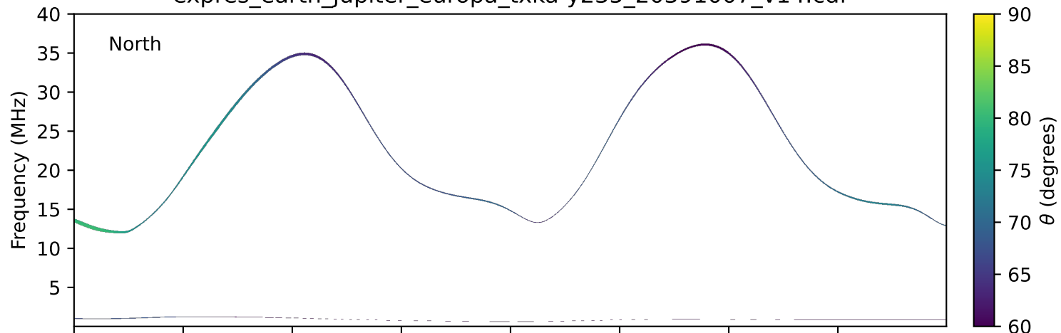
expres_earth_jupiter_europa_txka-y235_20391007_v14.cdf
