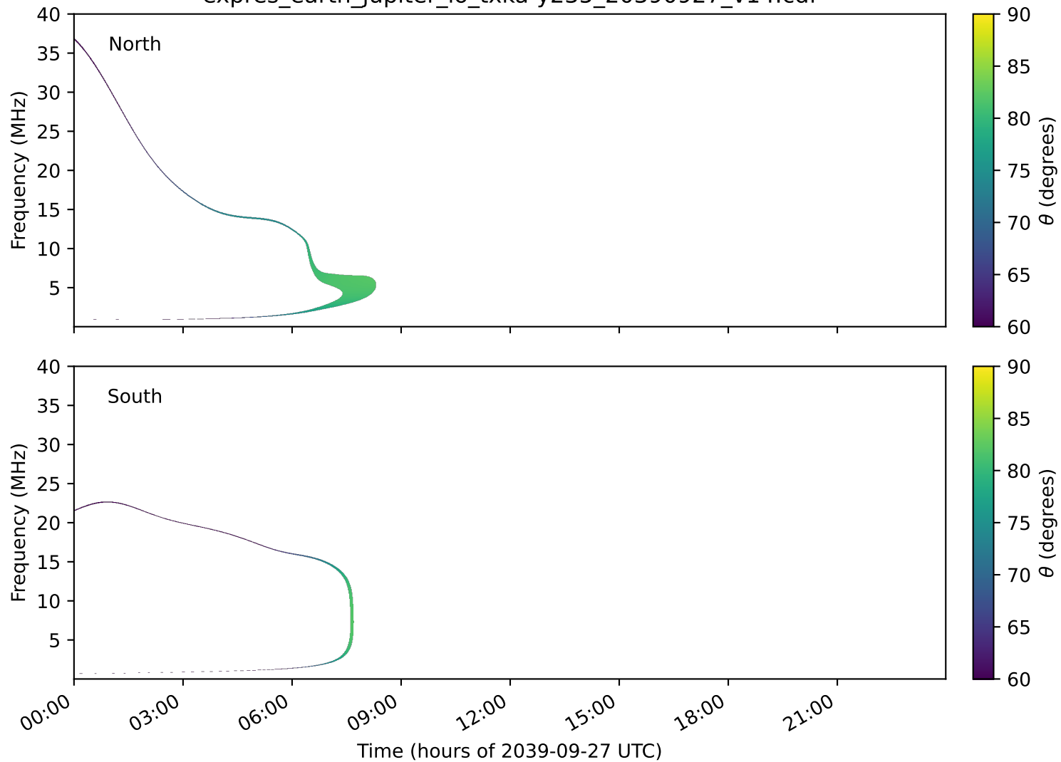
expres_earth_jupiter_io_txka-y235_20390927_v14.cdf
