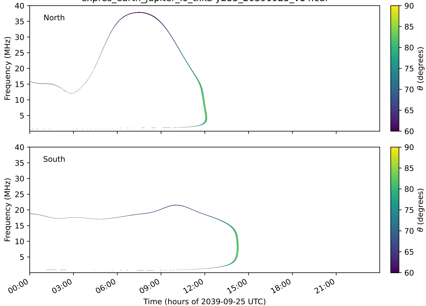
expres_earth_jupiter_io_txka-y235_20390925_v14.cdf
