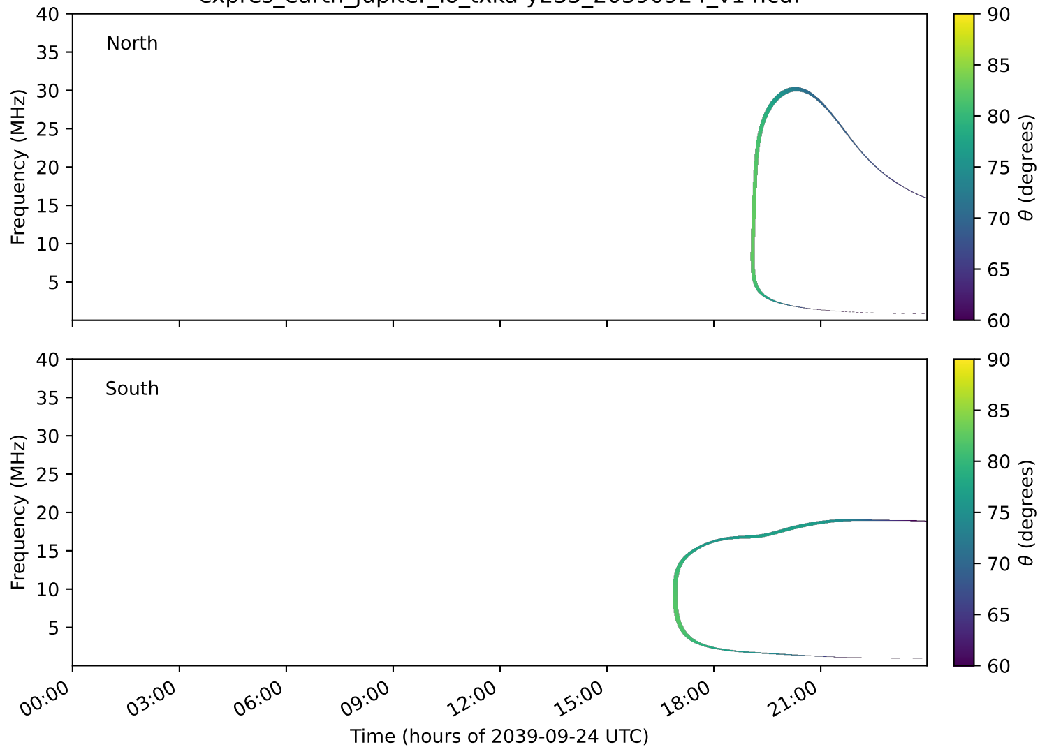
expres_earth_jupiter_io_txka-y235_20390924_v14.cdf
