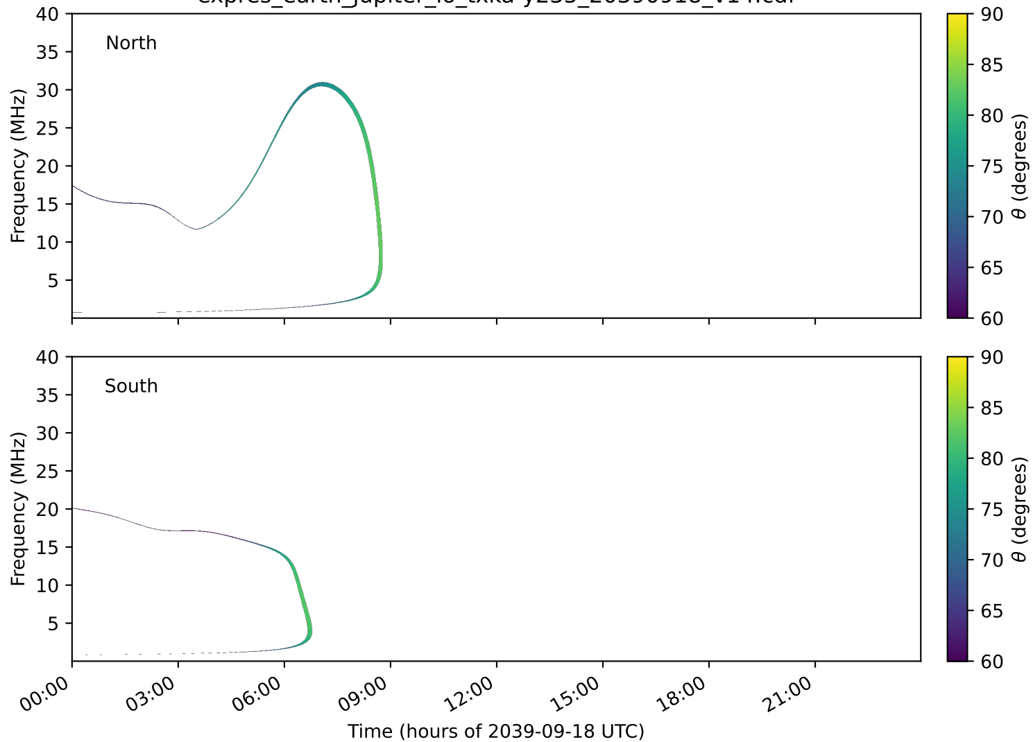
expres_earth_jupiter_io_txka-y235_20390918_v14.cdf
