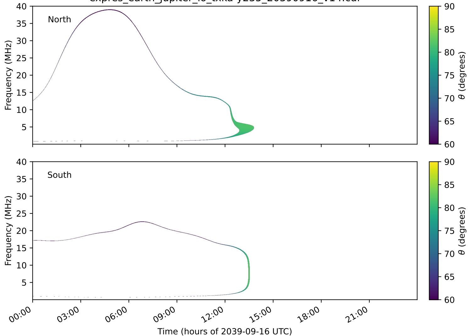
expres_earth_jupiter_io_txka-y235_20390916_v14.cdf
