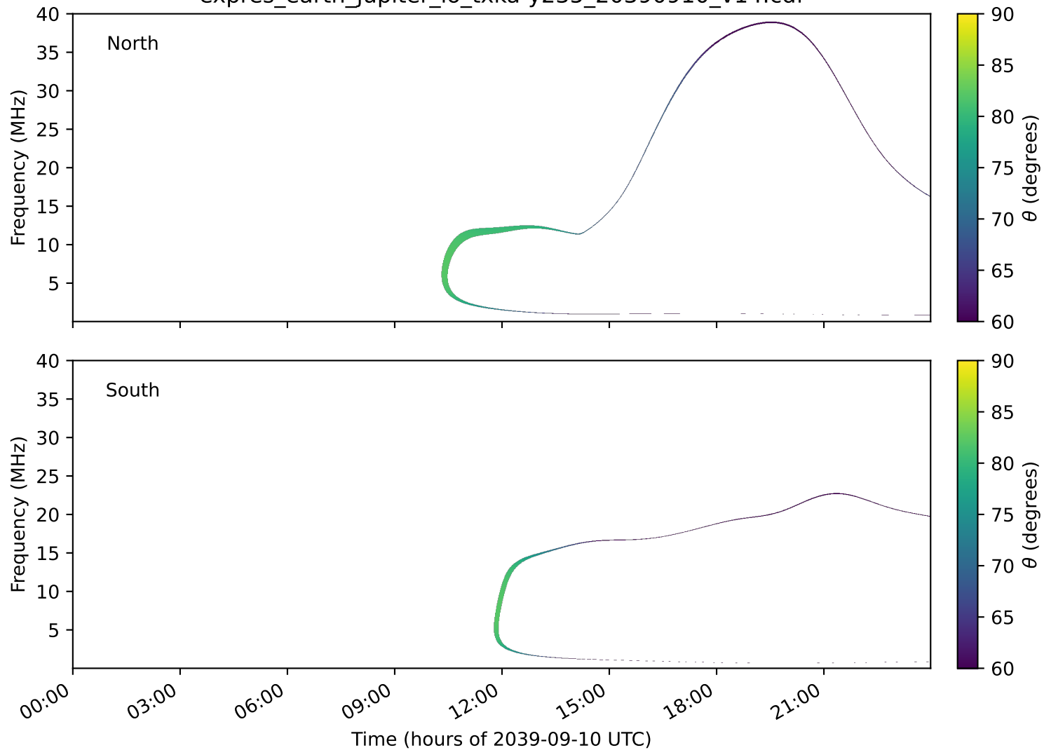
expres_earth_jupiter_io_txka-y235_20390910_v14.cdf
