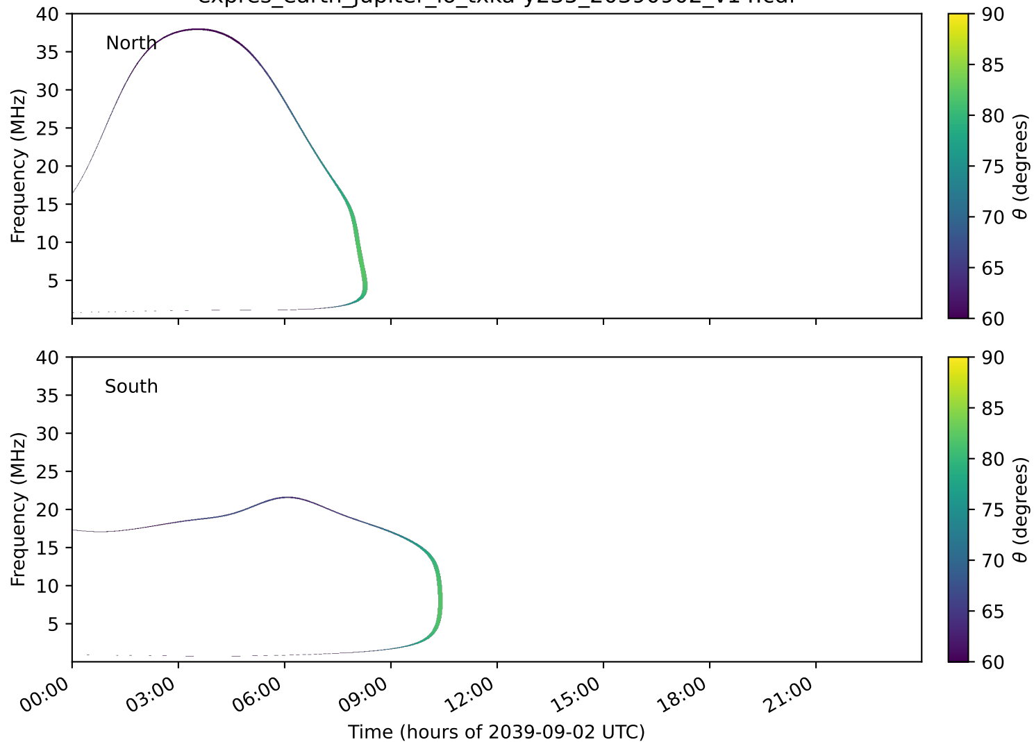
expres_earth_jupiter_io_txka-y235_20390902_v14.cdf
