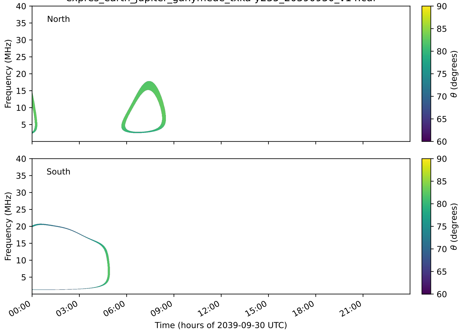
expres_earth_jupiter_ganymede_txka-y235_20390930_v14.cdf
