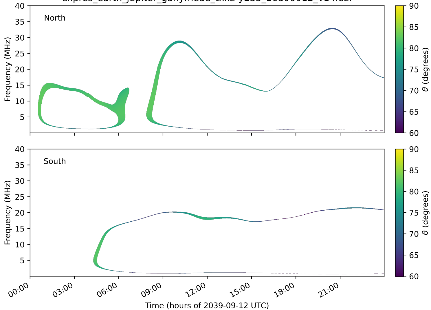
expres_earth_jupiter_ganymede_txka-y235_20390912_v14.cdf
