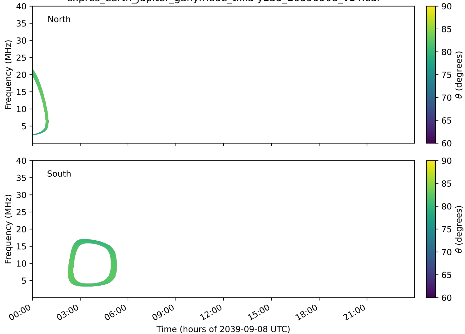
expres_earth_jupiter_ganymede_txka-y235_20390908_v14.cdf
