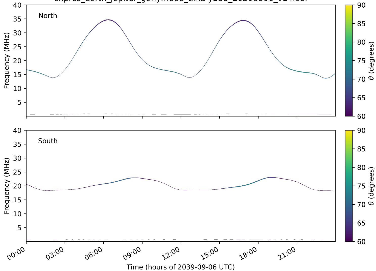
expres_earth_jupiter_ganymede_txka-y235_20390906_v14.cdf
