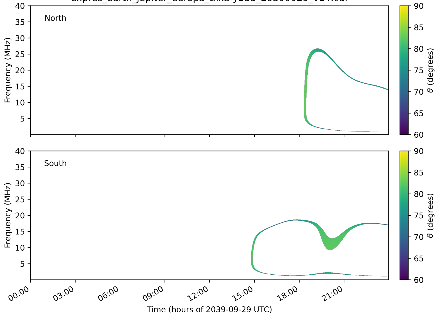
expres_earth_jupiter_europa_txka-y235_20390929_v14.cdf
