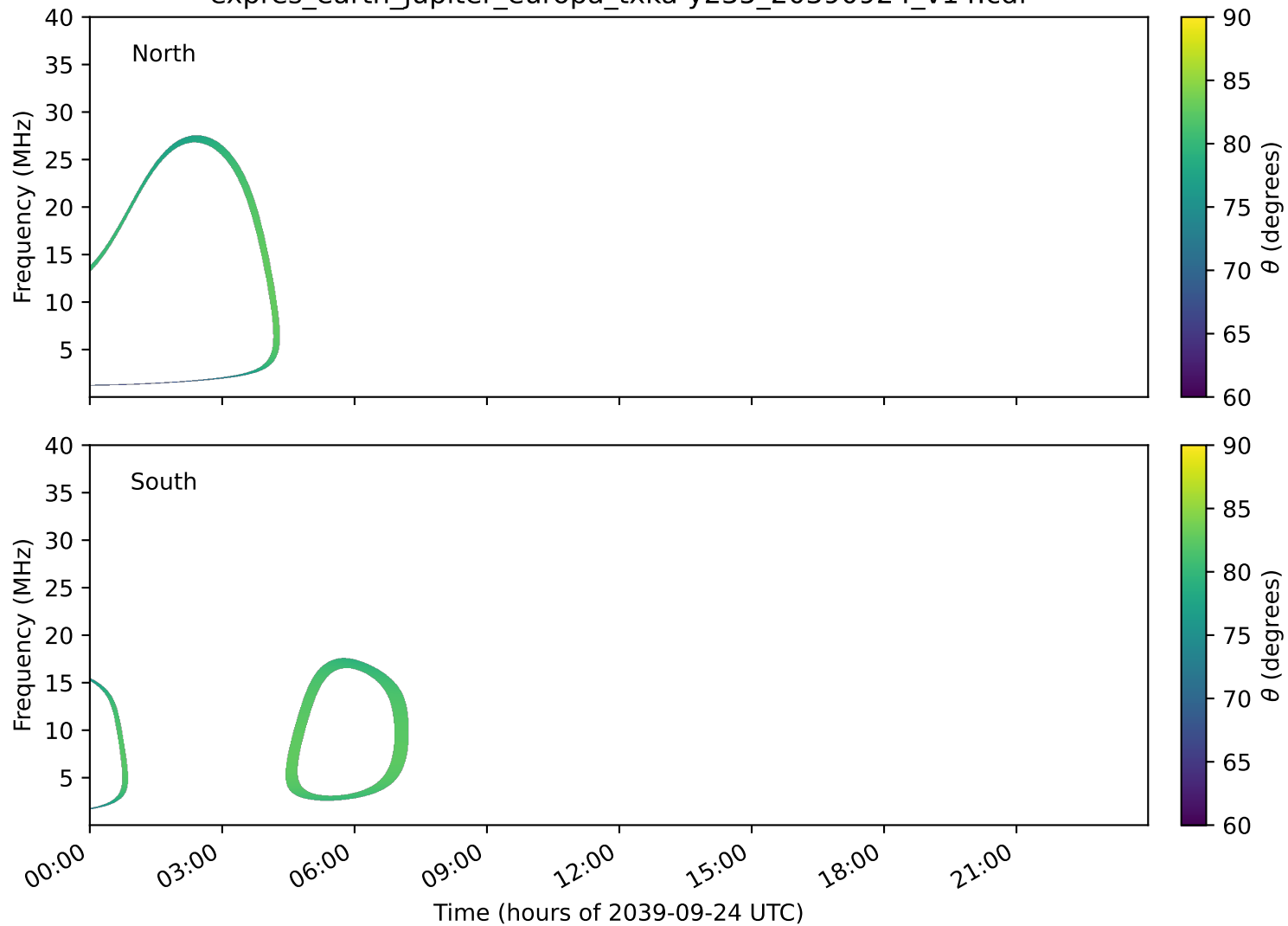
expres_earth_jupiter_europa_txka-y235_20390924_v14.cdf
