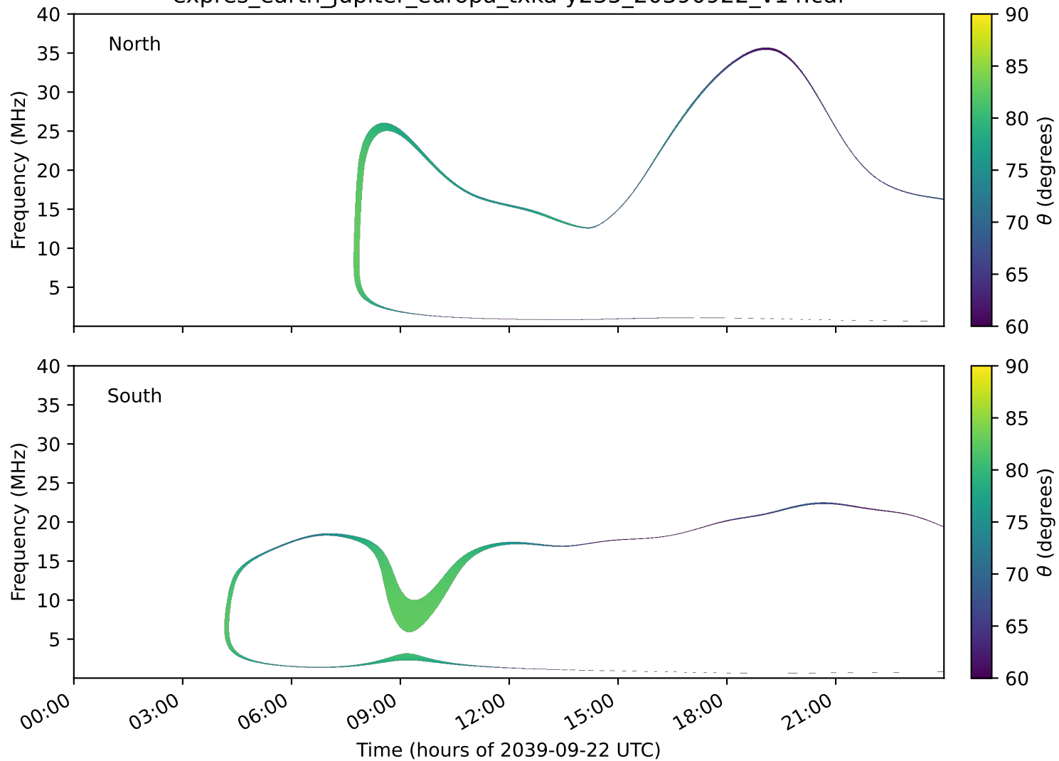
expres_earth_jupiter_europa_txka-y235_20390922_v14.cdf
