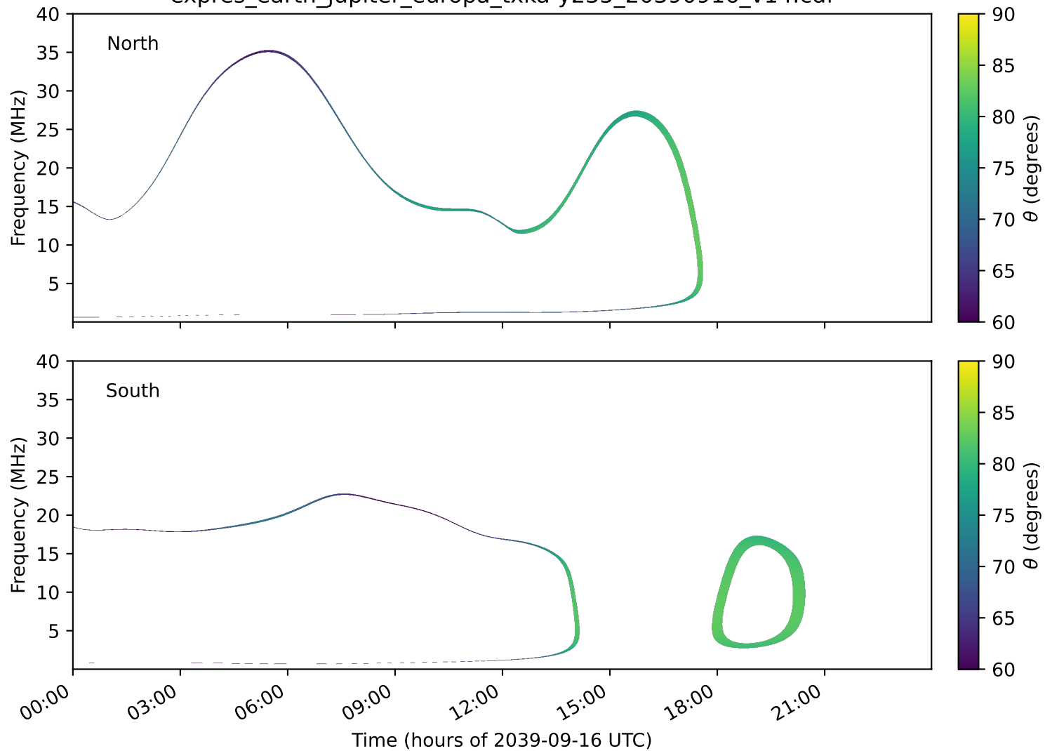
expres_earth_jupiter_europa_txka-y235_20390916_v14.cdf
