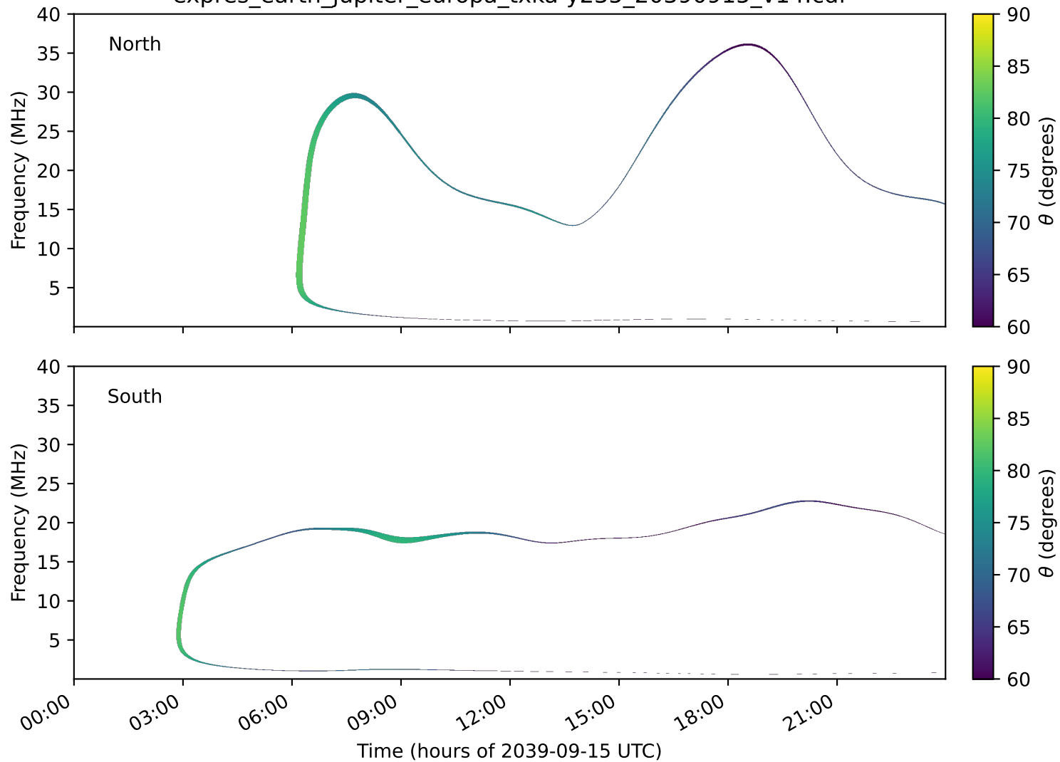
expres_earth_jupiter_europa_txka-y235_20390915_v14.cdf
