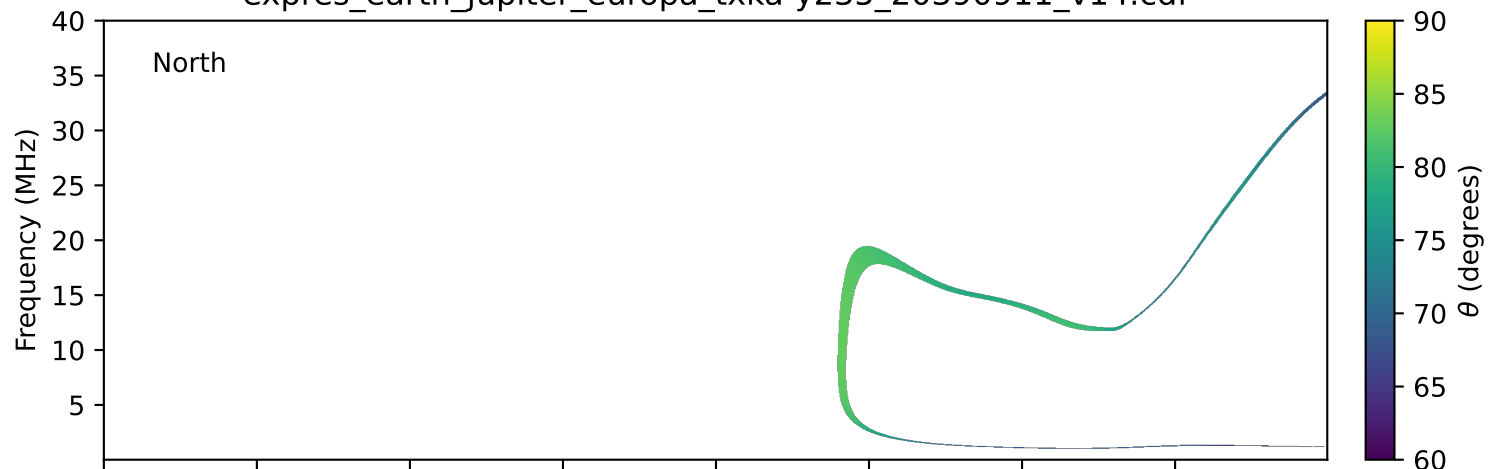
expres_earth_jupiter_europa_txka-y235_20390911_v14.cdf
