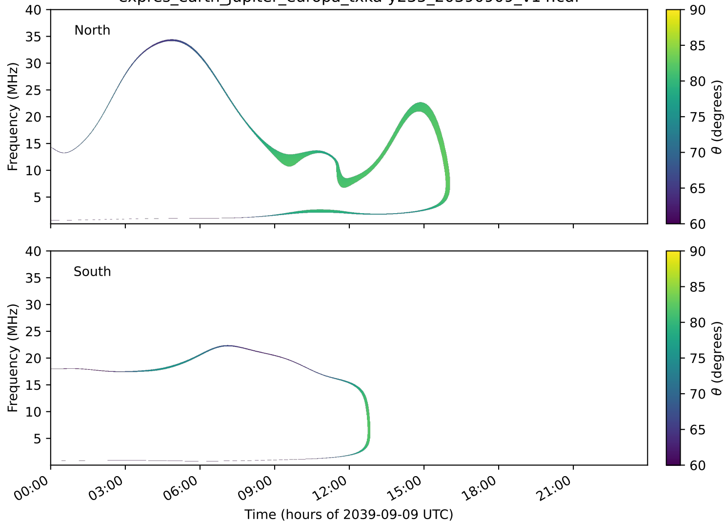
expres_earth_jupiter_europa_txka-y235_20390909_v14.cdf
