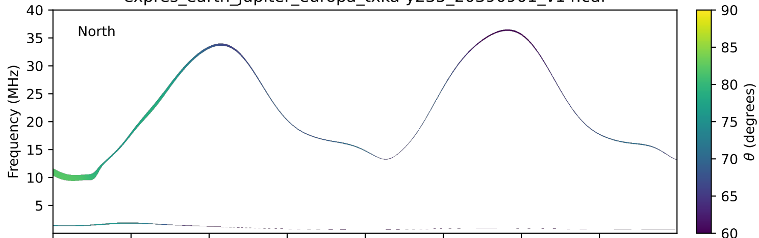
expres_earth_jupiter_europa_txka-y235_20390901_v14.cdf
