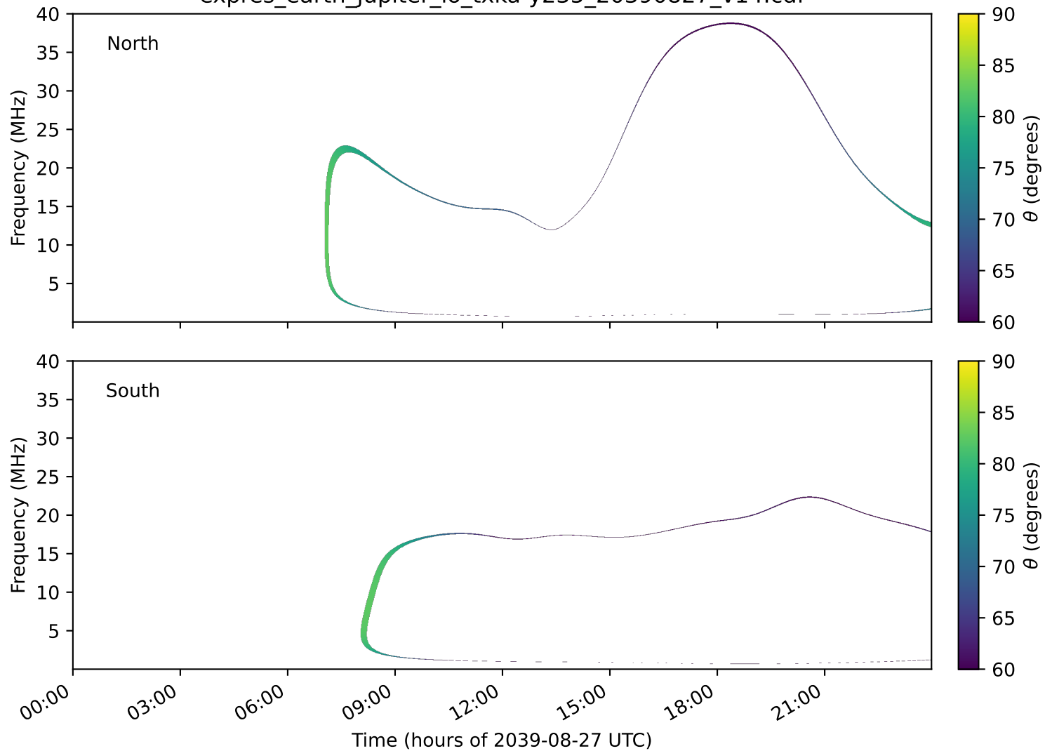
expres_earth_jupiter_io_txka-y235_20390827_v14.cdf
