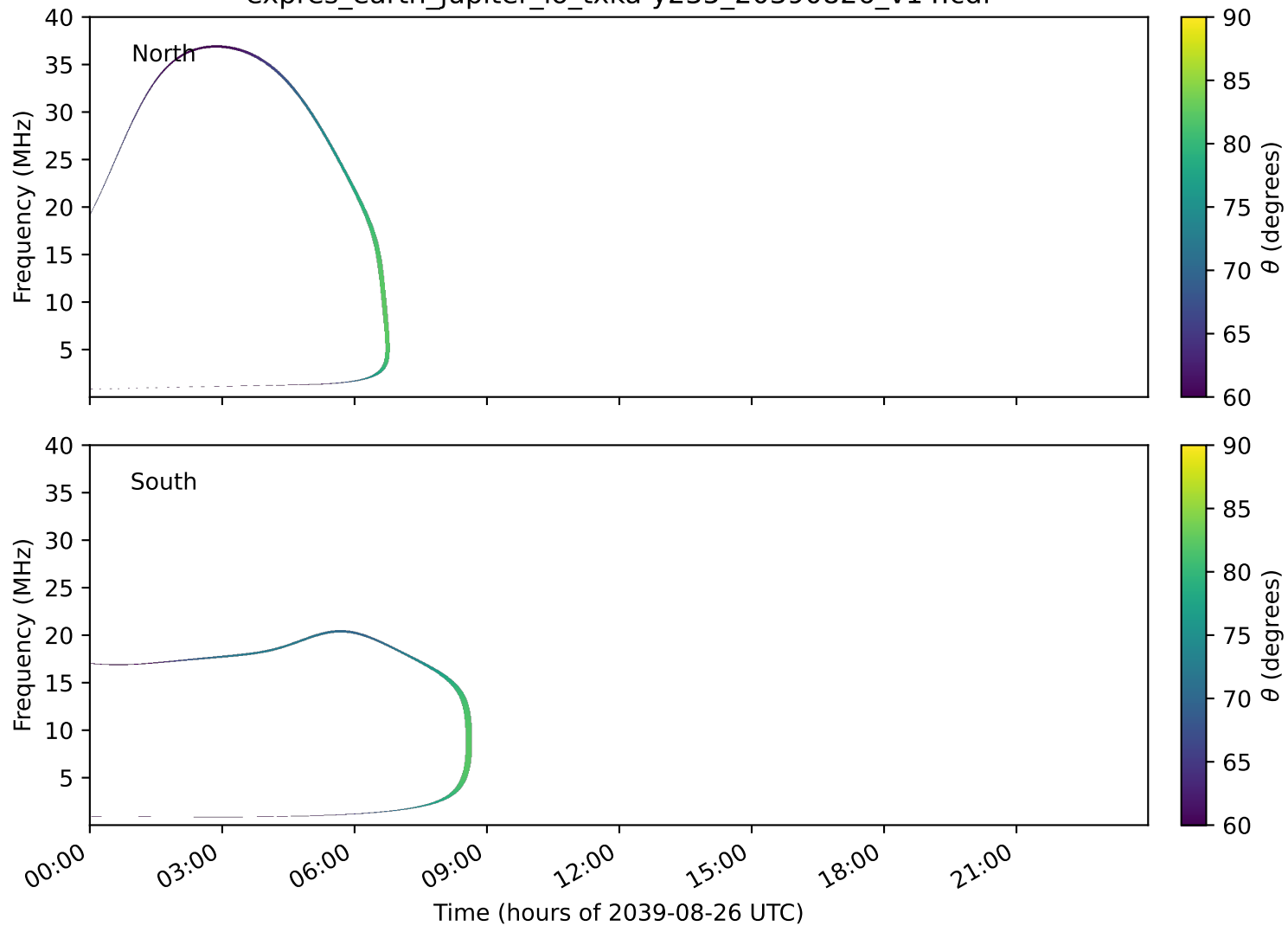
expres_earth_jupiter_io_txka-y235_20390826_v14.cdf
