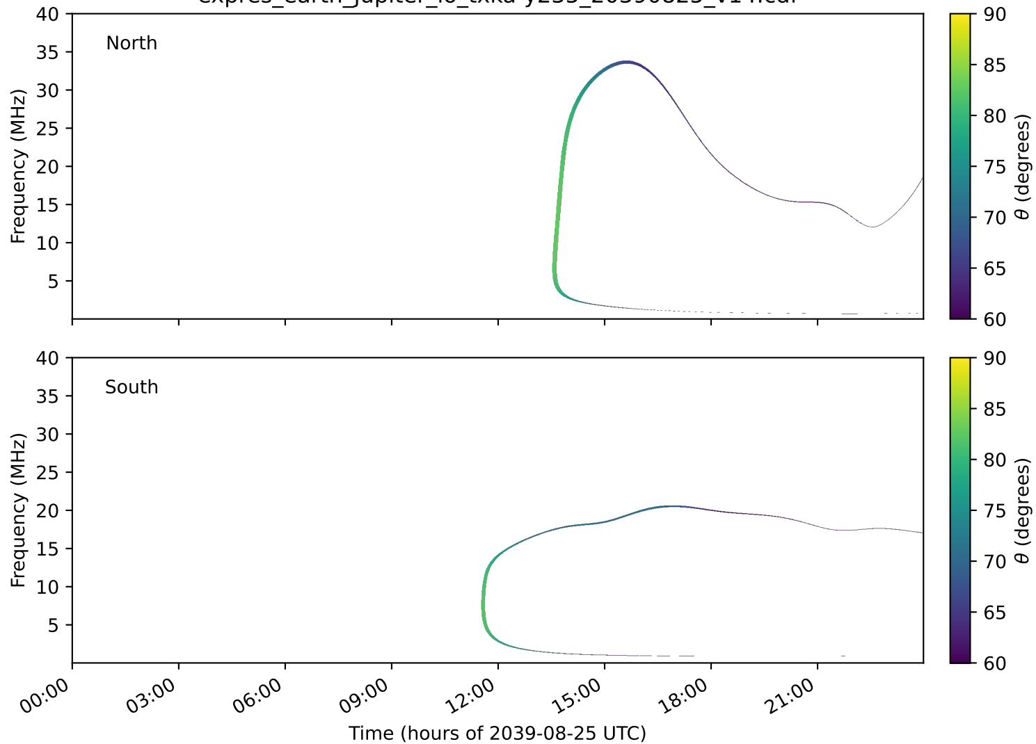
expres_earth_jupiter_io_txka-y235_20390825_v14.cdf
