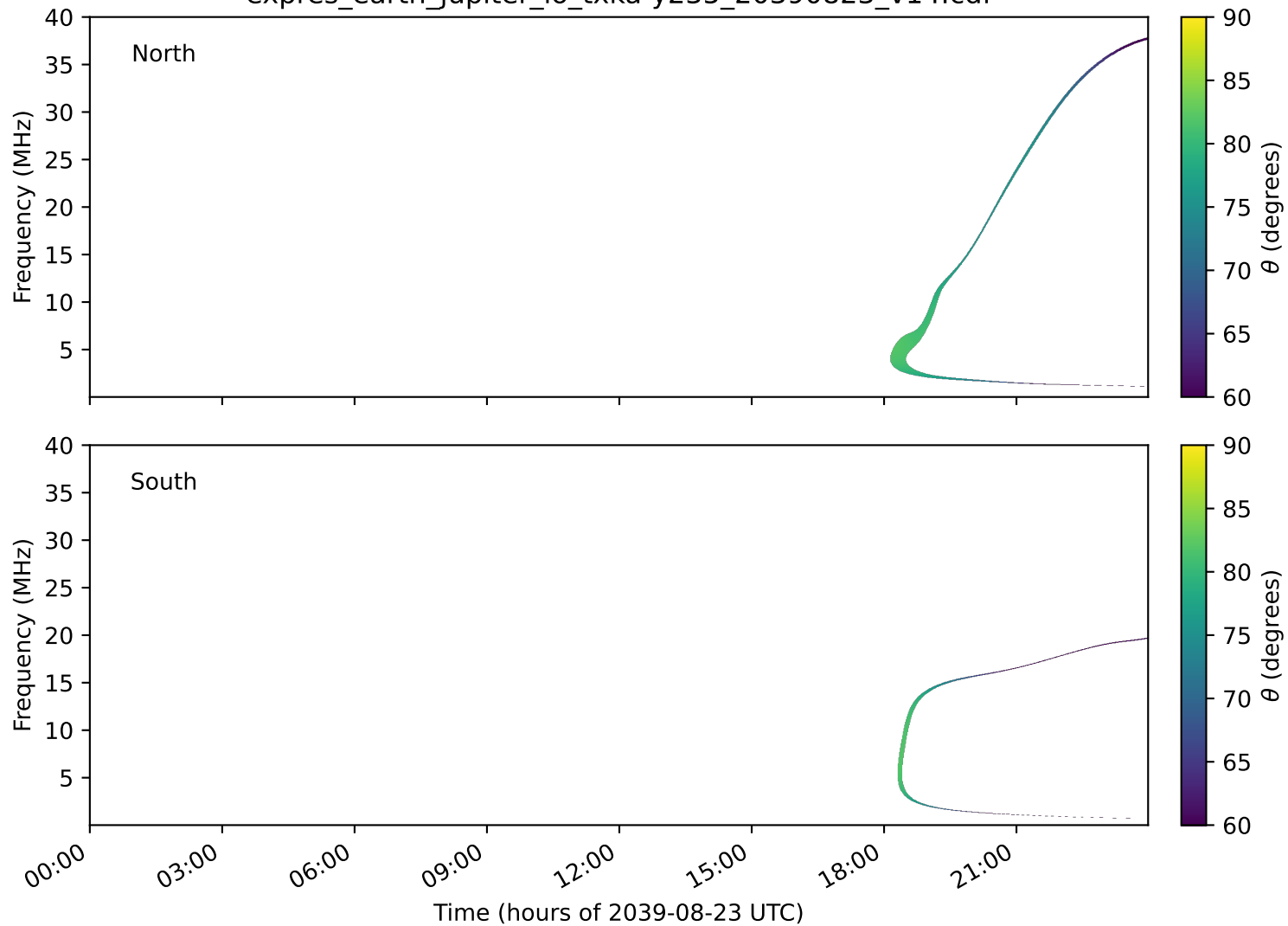
expres_earth_jupiter_io_txka-y235_20390823_v14.cdf
