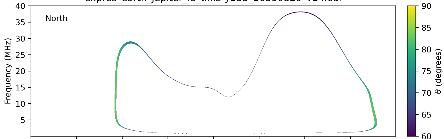
expres_earth_jupiter_io_txka-y235_20390820_v14.cdf
