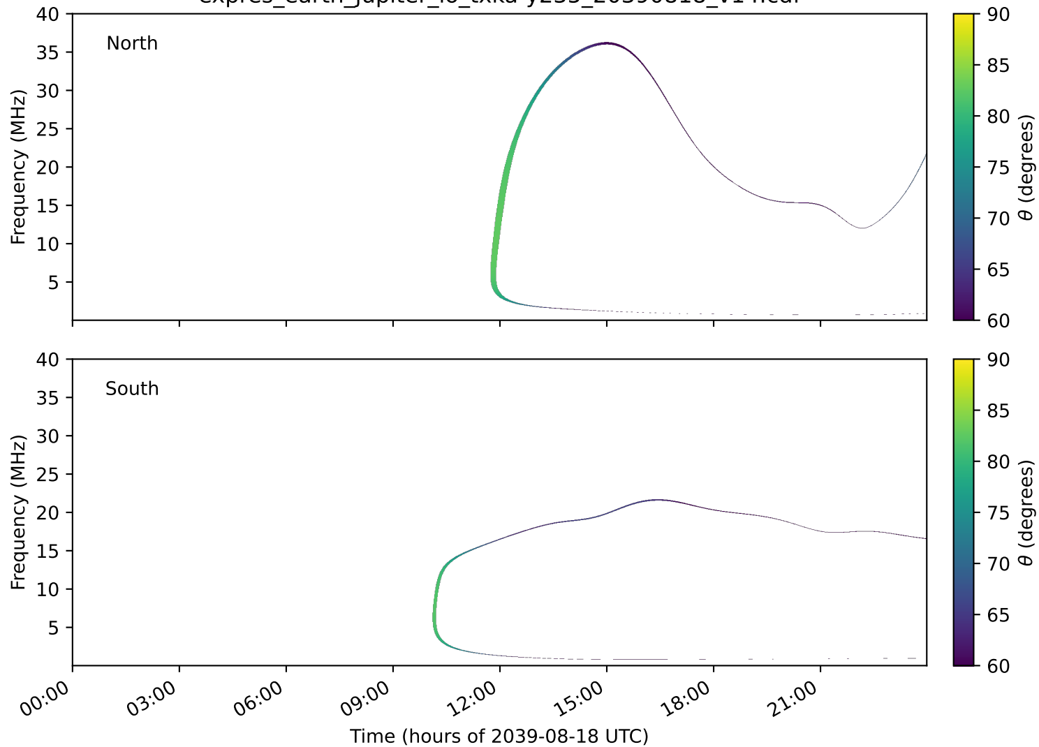
expres_earth_jupiter_io_txka-y235_20390818_v14.cdf
