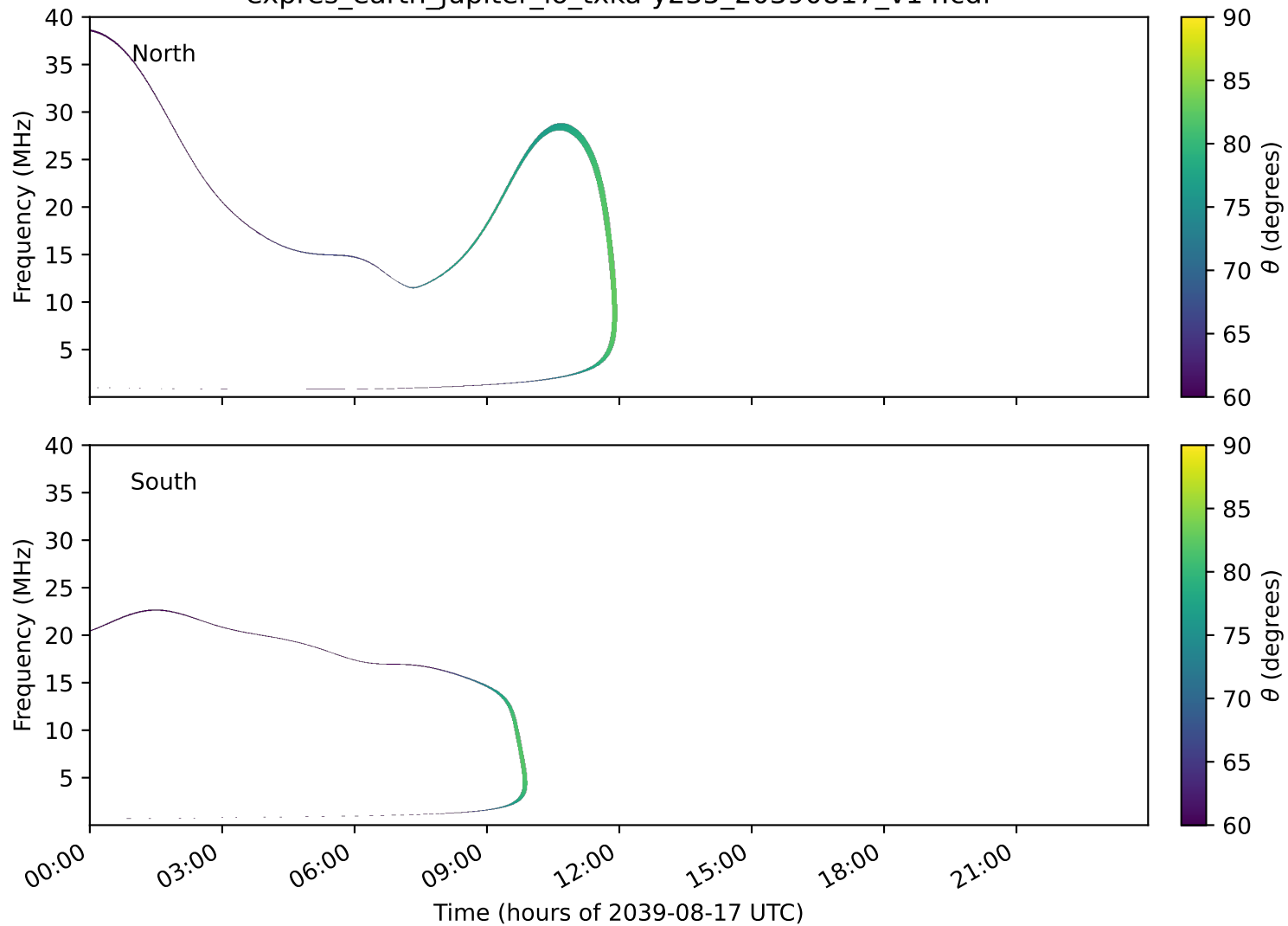
expres_earth_jupiter_io_txka-y235_20390817_v14.cdf
