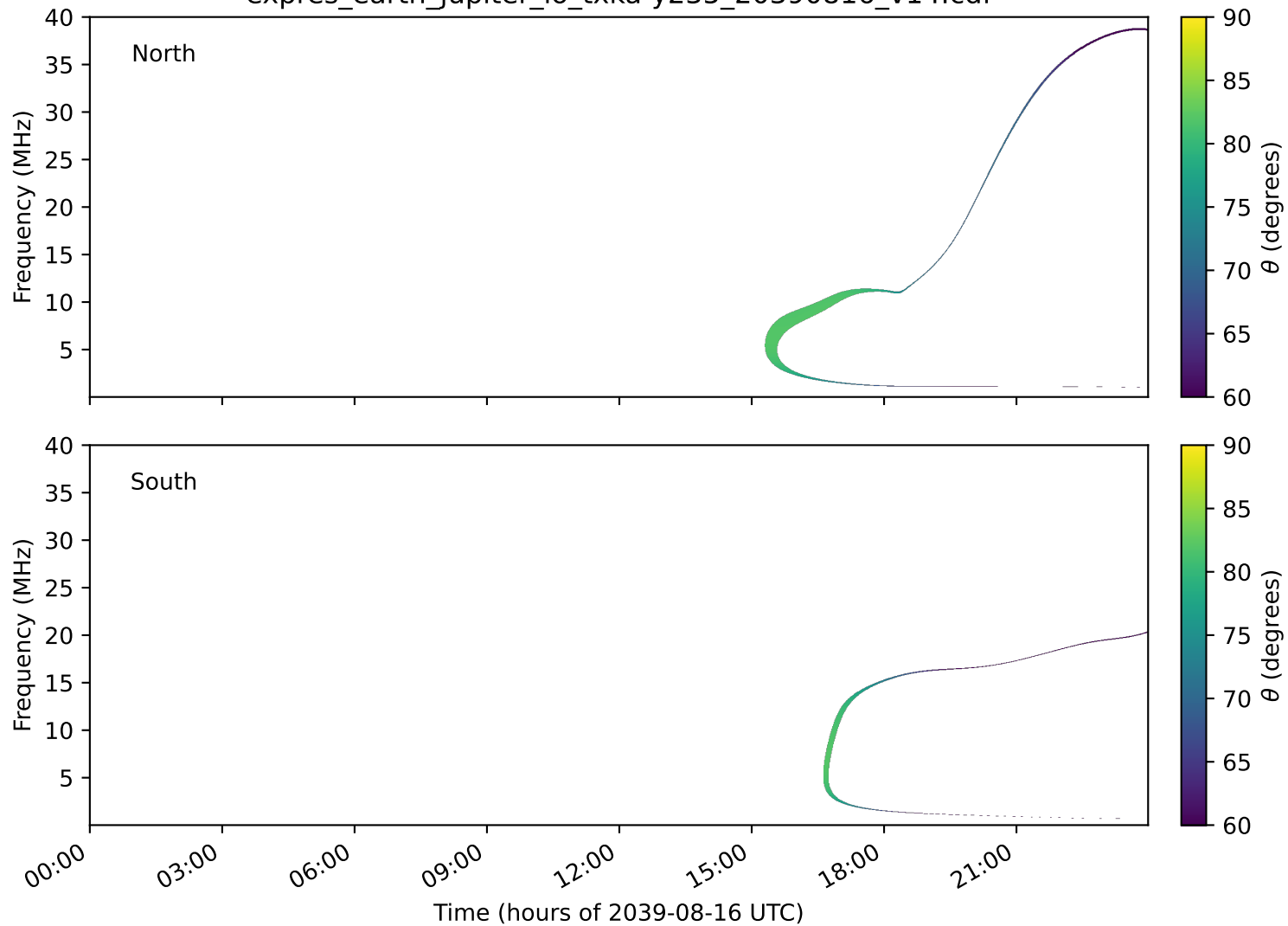
expres_earth_jupiter_io_txka-y235_20390816_v14.cdf
