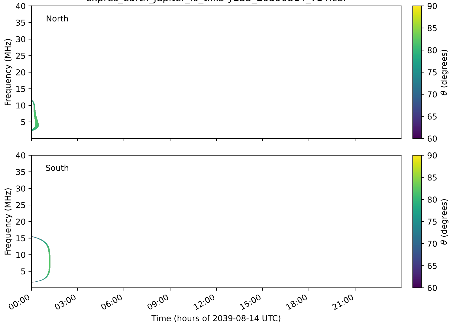
expres_earth_jupiter_io_txka-y235_20390814_v14.cdf
