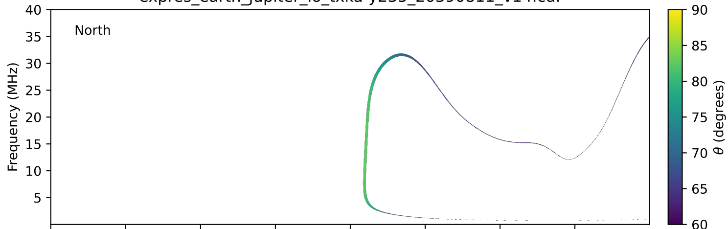
expres_earth_jupiter_io_txka-y235_20390811_v14.cdf
