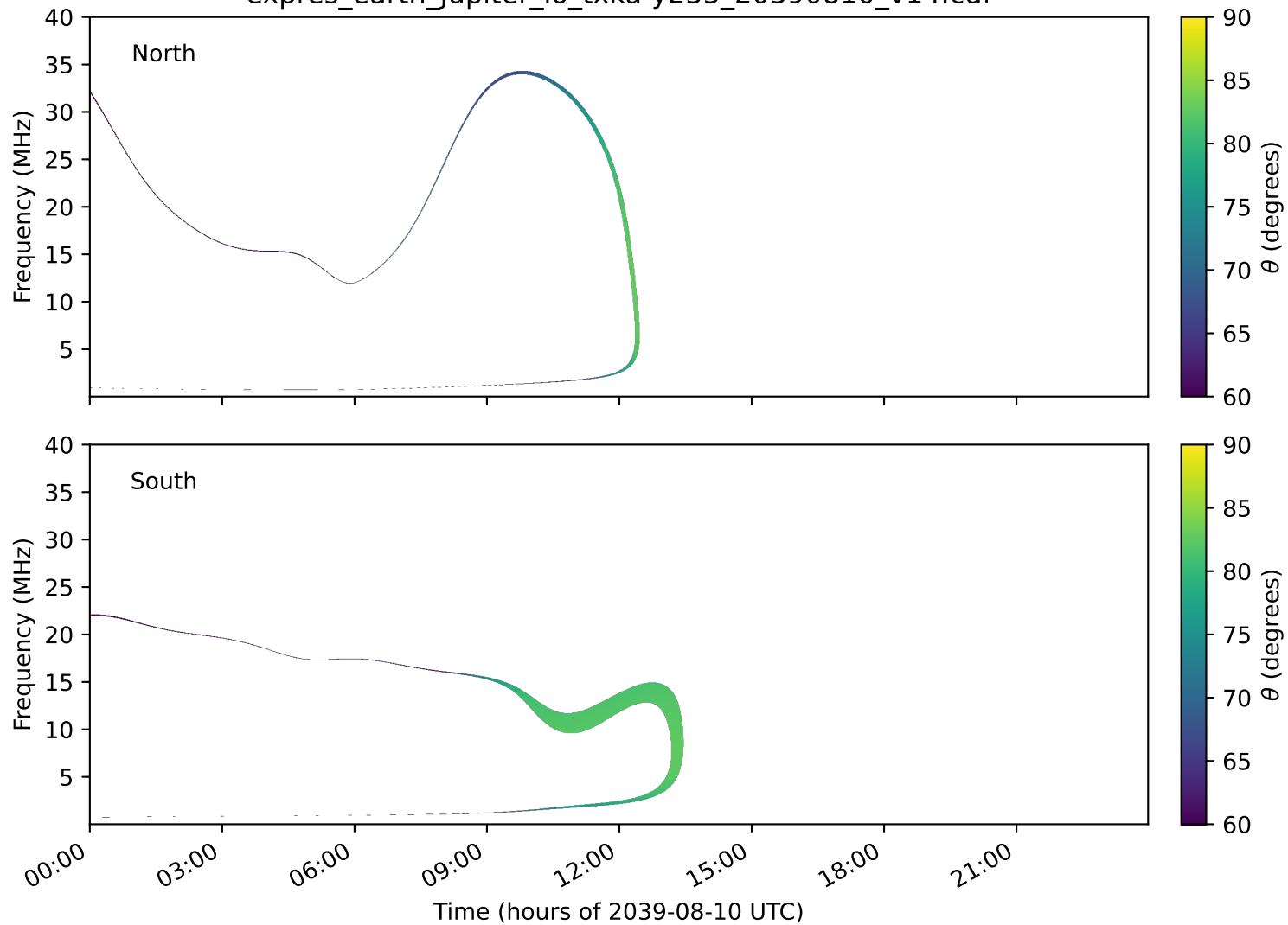
expres_earth_jupiter_io_txka-y235_20390810_v14.cdf
