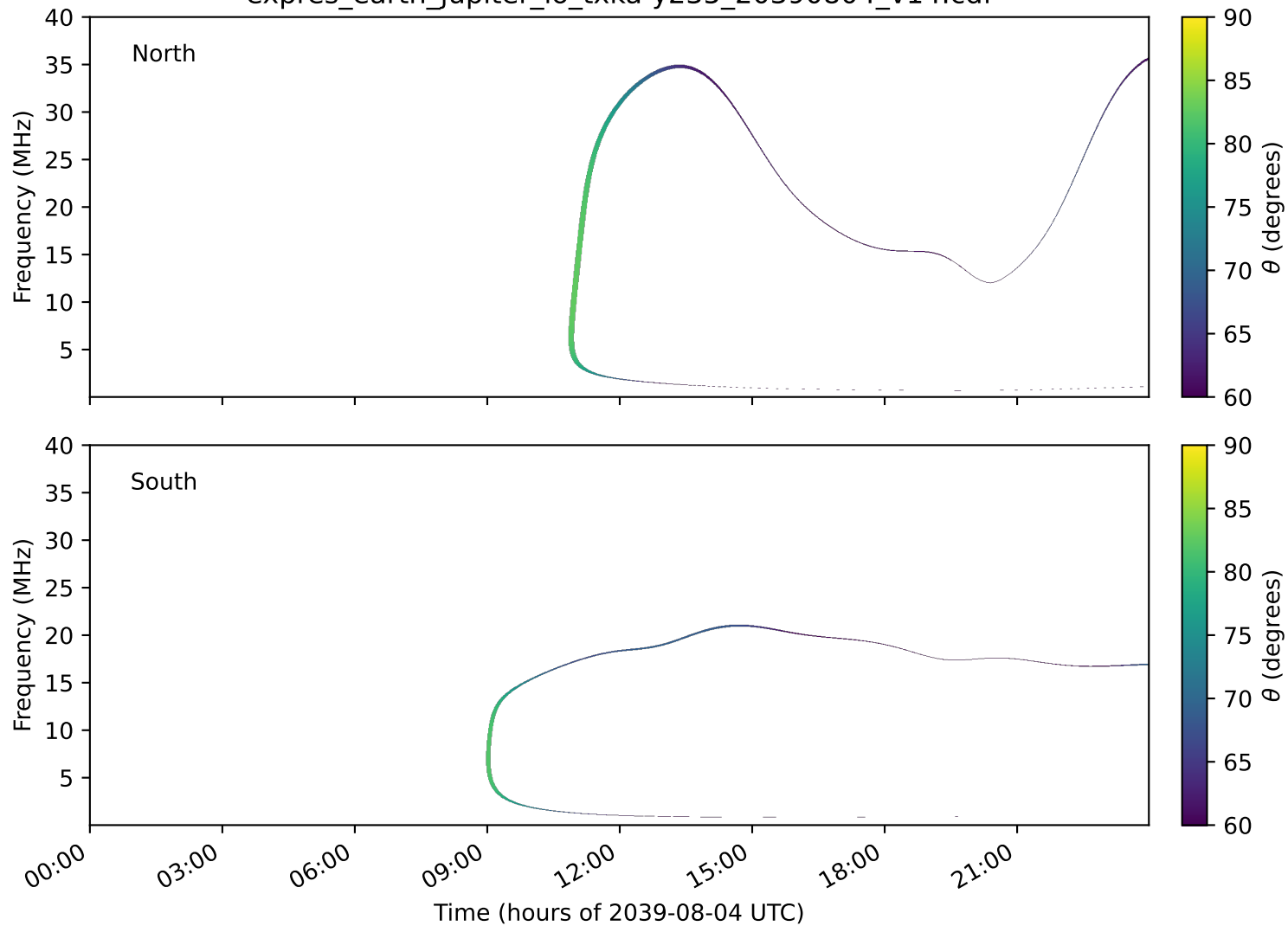
expres_earth_jupiter_io_txka-y235_20390804_v14.cdf
