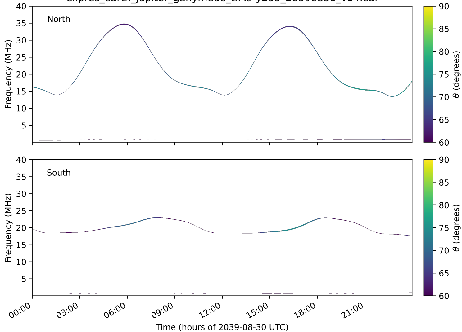
expres_earth_jupiter_ganymede_txka-y235_20390830_v14.cdf
