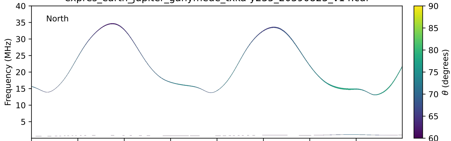
expres_earth_jupiter_ganymede_txka-y235_20390823_v14.cdf
