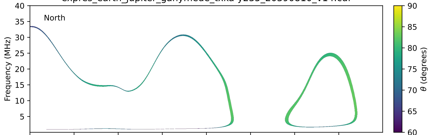
expres_earth_jupiter_ganymede_txka-y235_20390810_v14.cdf
