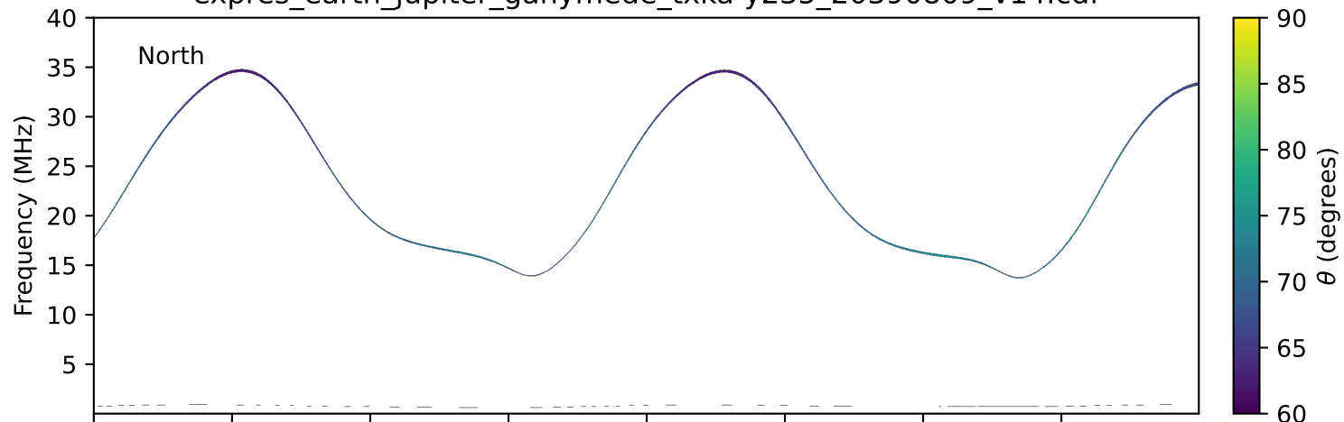
expres_earth_jupiter_ganymede_txka-y235_20390809_v14.cdf
