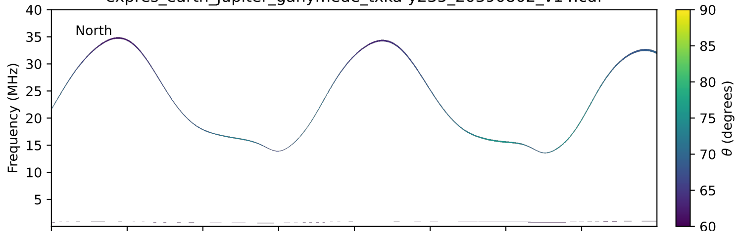
expres_earth_jupiter_ganymede_txka-y235_20390802_v14.cdf
