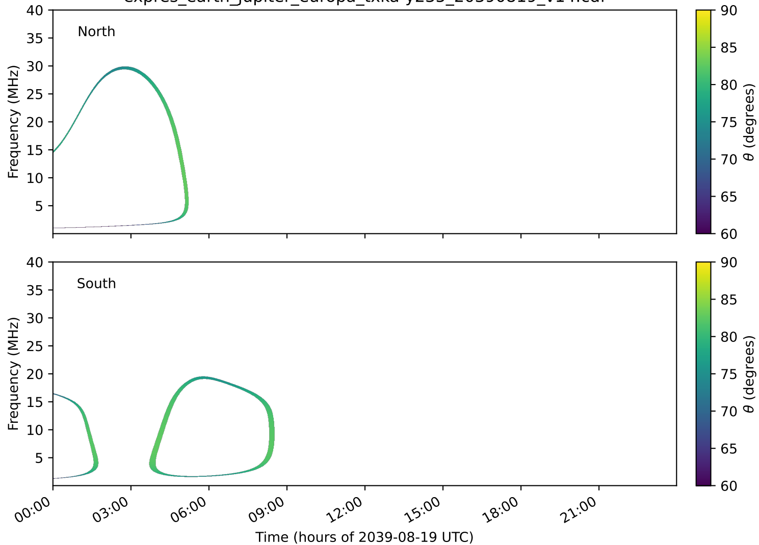
expres_earth_jupiter_europa_txka-y235_20390819_v14.cdf
