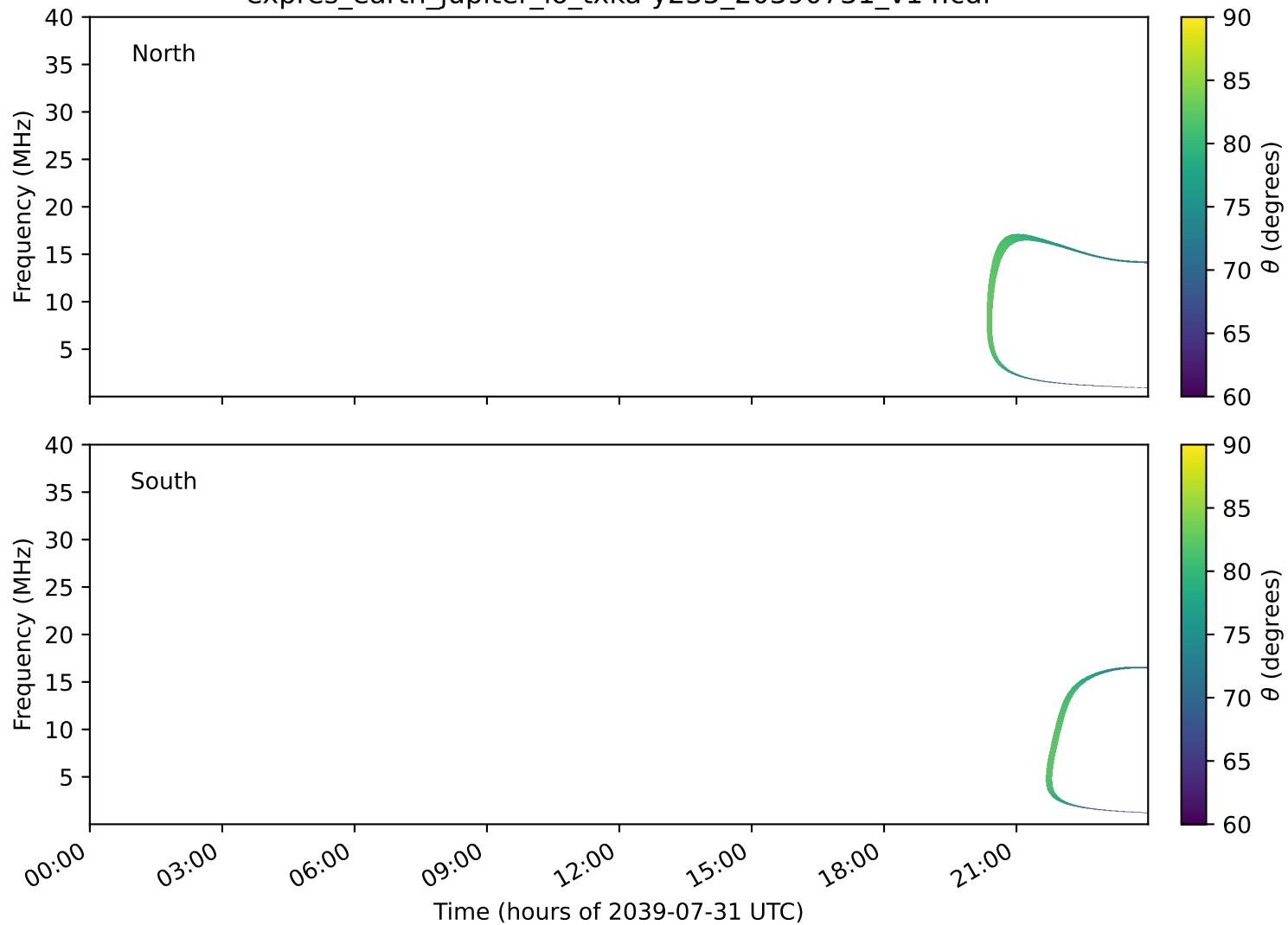
expres_earth_jupiter_io_txka-y235_20390731_v14.cdf
