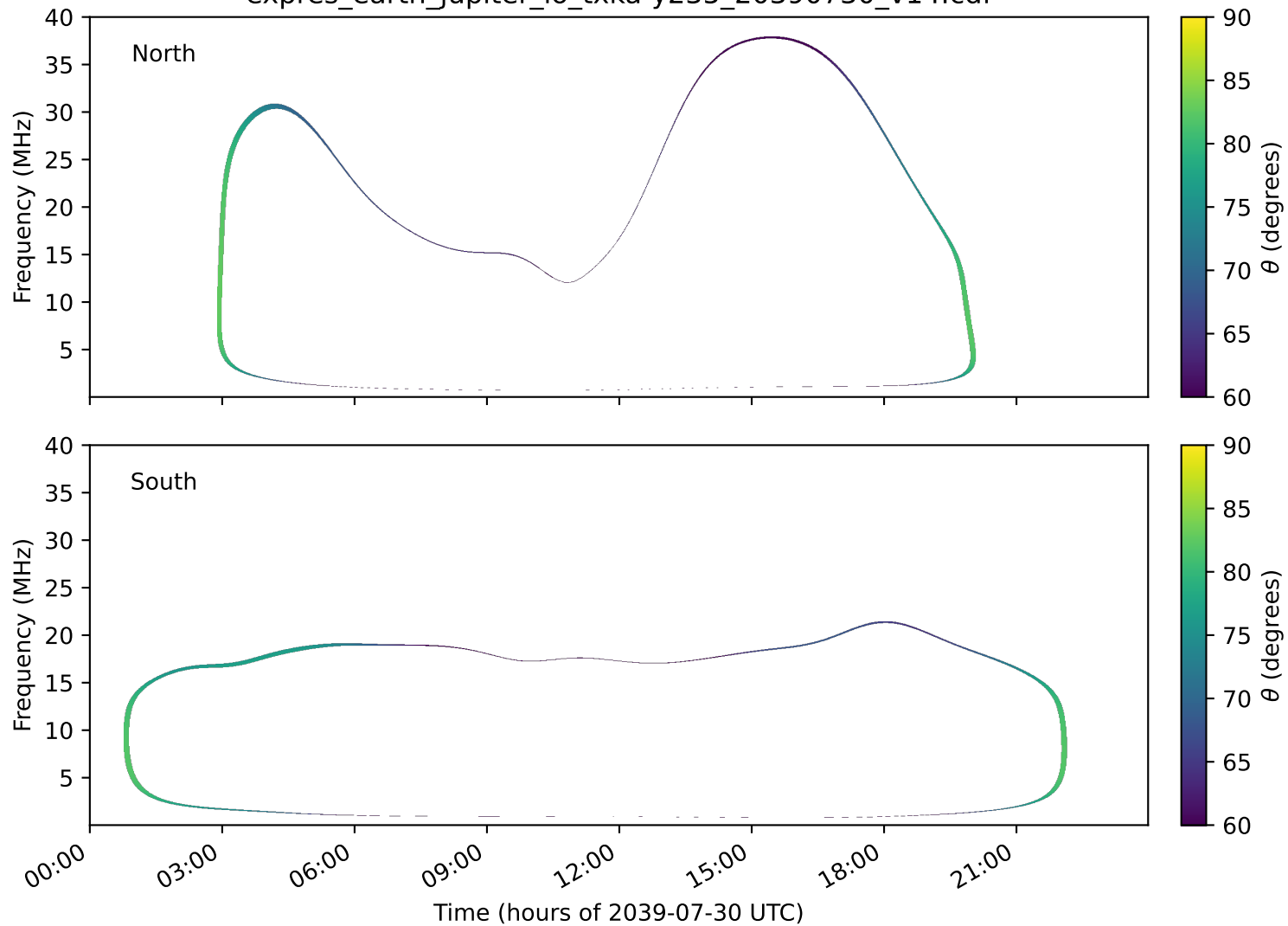
expres_earth_jupiter_io_txka-y235_20390730_v14.cdf
